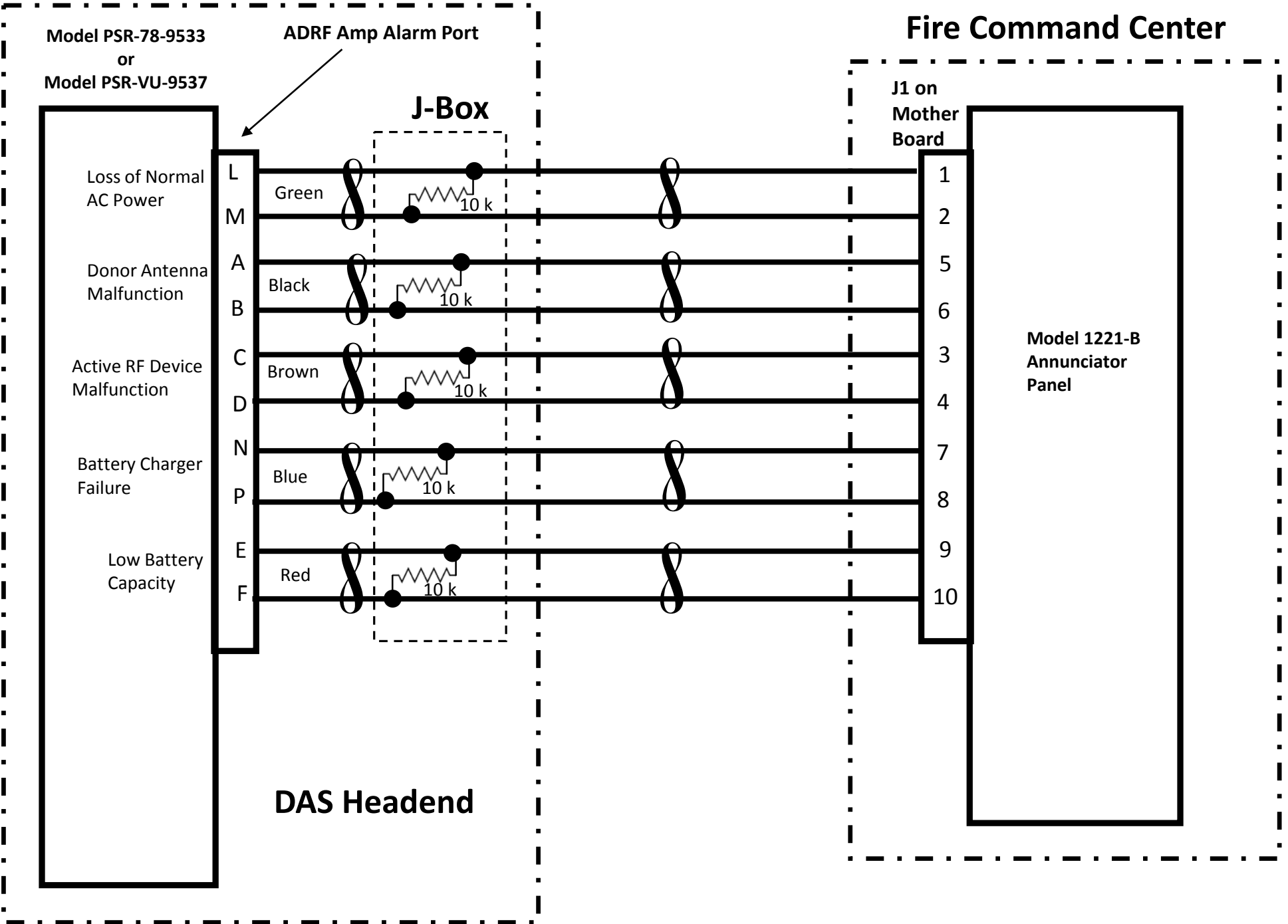
ADRF Amplifier Interface Drawing
